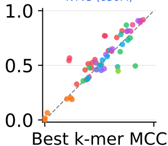
NTv3 (650M)
