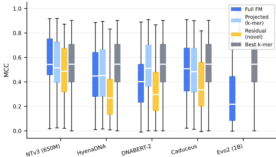
(b) Downstream classification performance
