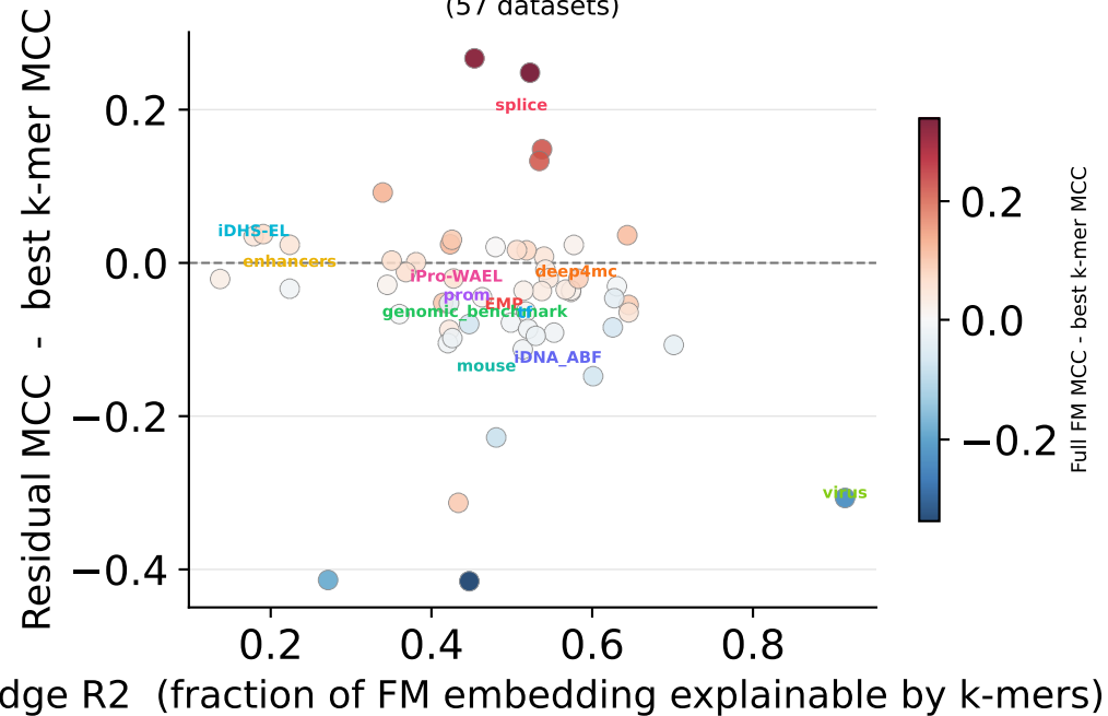
NTv3 (k=6): k-mer Explainability vs. Residual Value (57 datasets)
