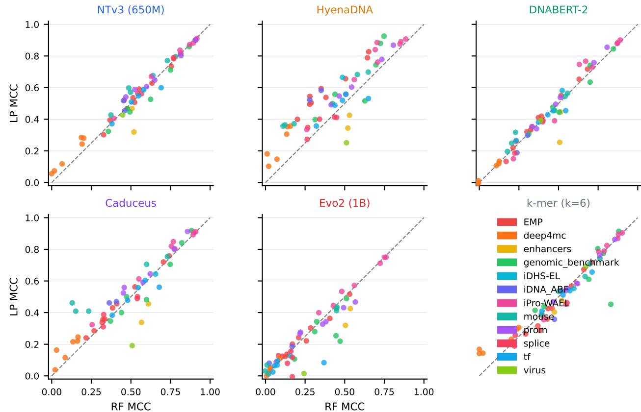
Supplementary Figure S1: Random Forest vs. Linear Probe Classifier
