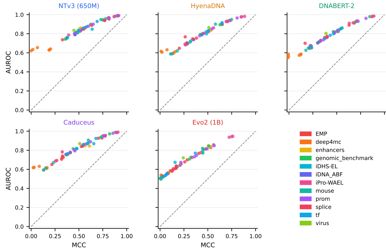
Supplementary Figure S2: AUROC vs MCC Metric Consistency
