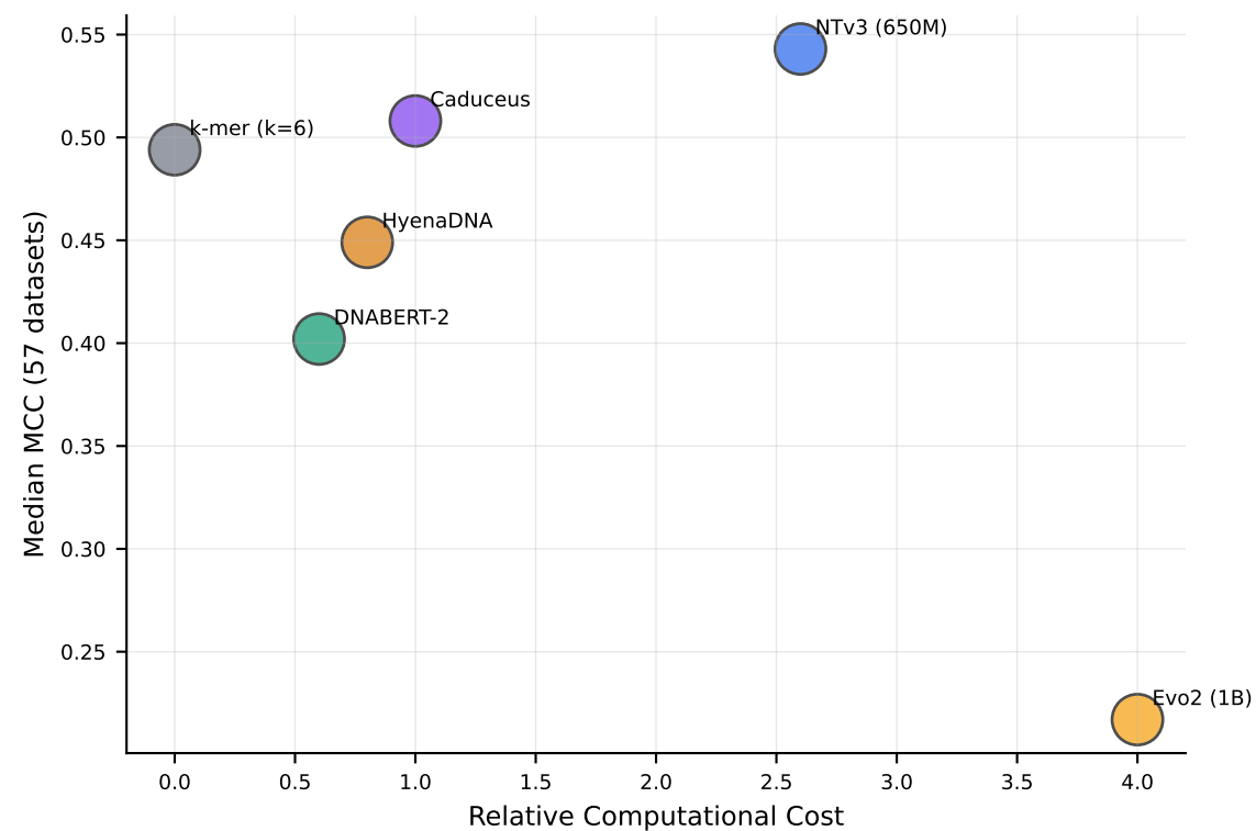
Cost-Benefit Tradeoff
