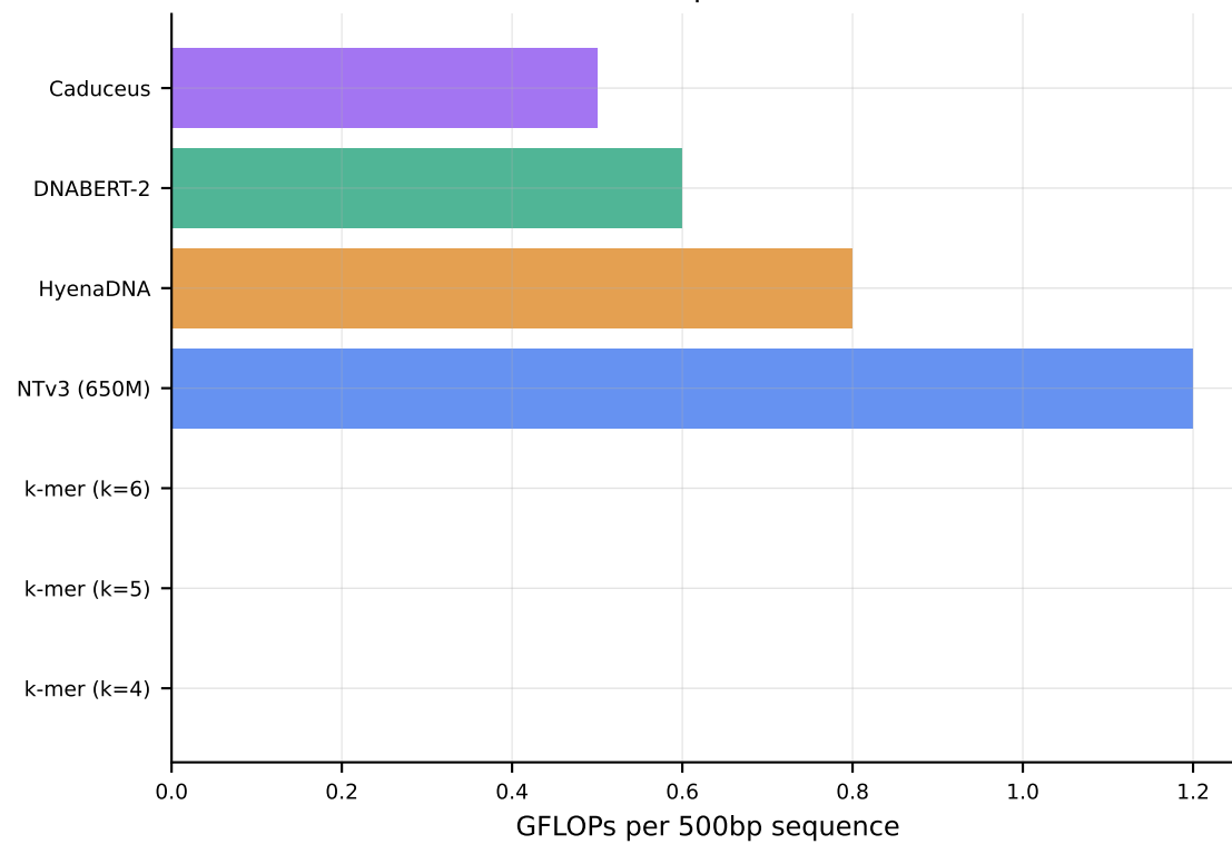
Cost-Benefit Tradeoff
