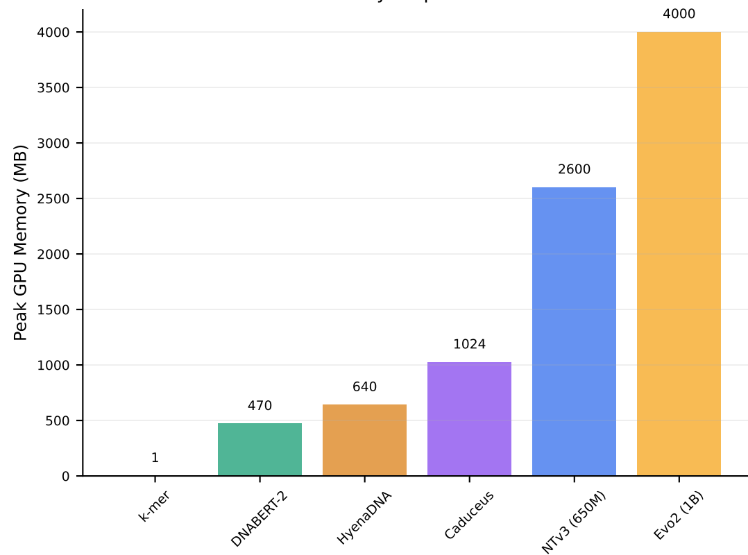
Memory Requirements
