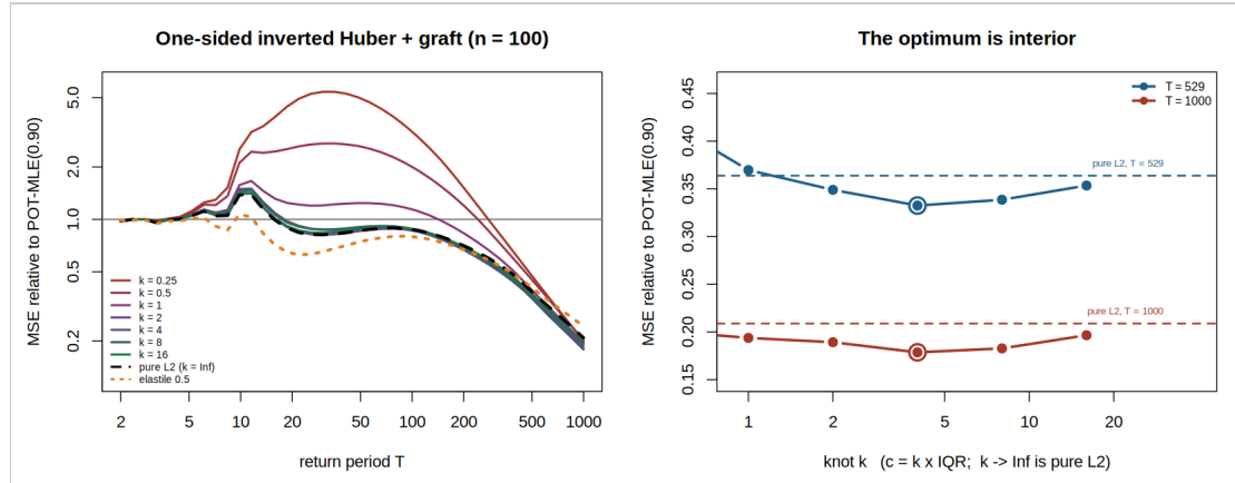
Figure 2. The knot sweep under misspecification. Left, MSE relative to peaks-over-threshold against return period for knots k = 0.25 to 16 , with pure L2 (the k \rightarrow \infty limit) dashed and the \alpha = 0.5 elastic dotted. Small knots are catastrophic below T = 200 , the mechanism being Section 3.3. Right, the same numbers read along k : the optimum is interior at k = 4 , circled, and the curve turns back towards the pure-L2 line on both sides.
