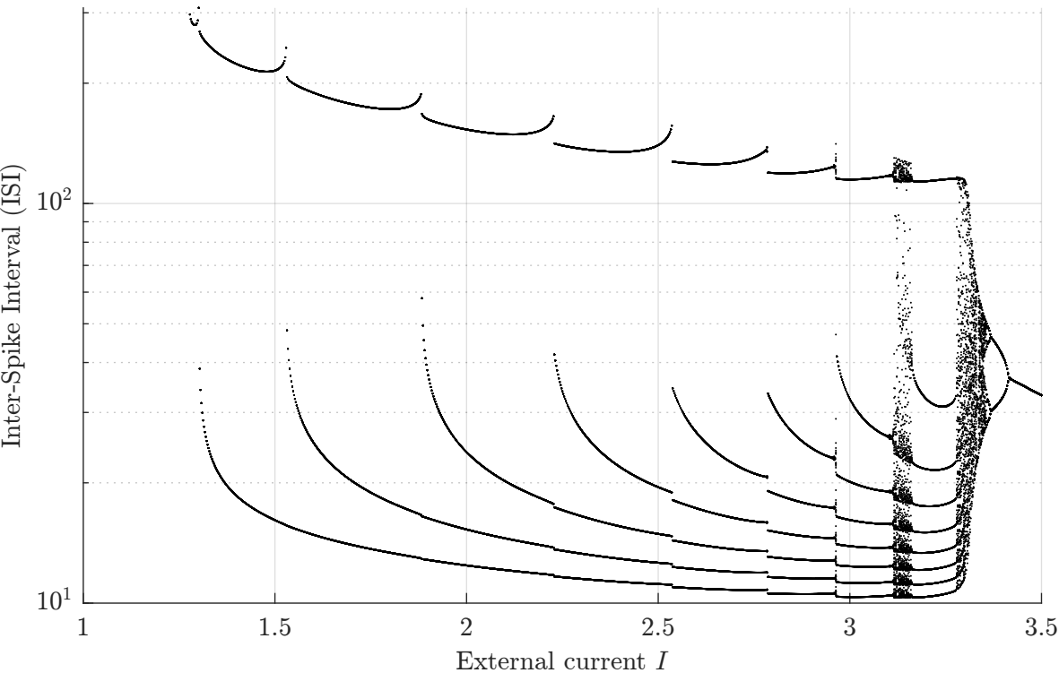
Bifurcation Diagram I vs ISI
