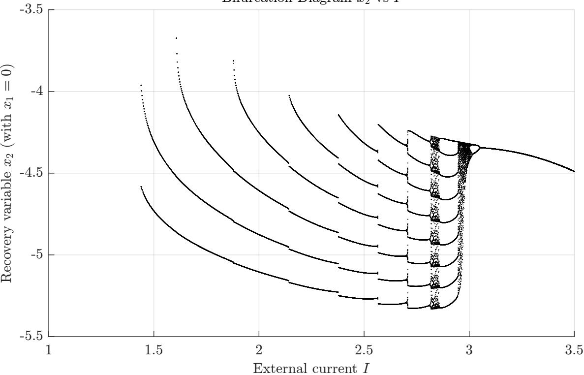
Bifurcation Diagram x_2 vs I
