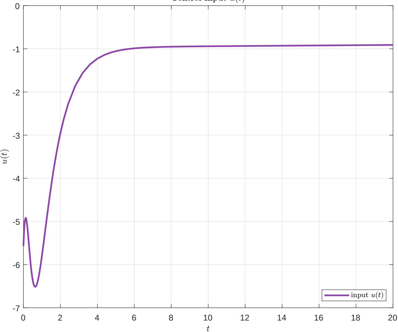
Control Input u(t)
