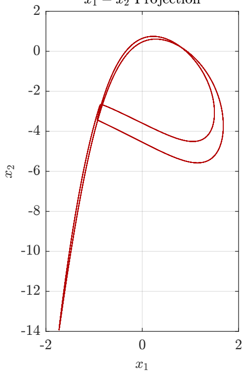
x_1 - x_2 Projection
