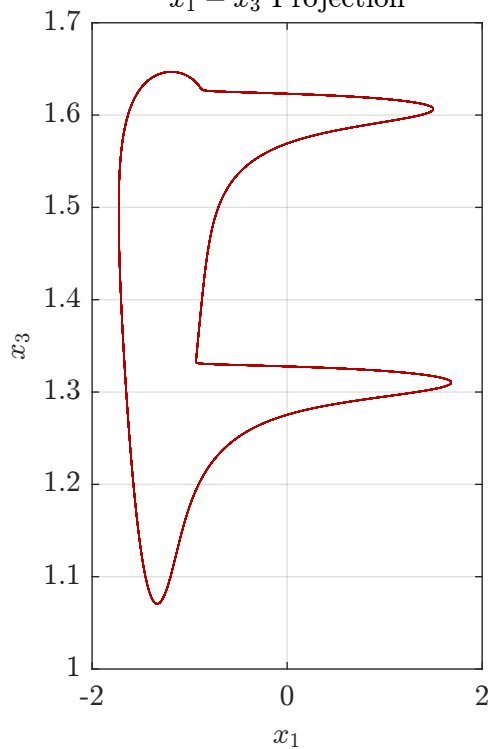
x_1 - x_3 Projection
