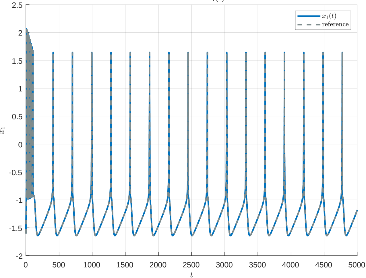
Reference vs x_1(t)
