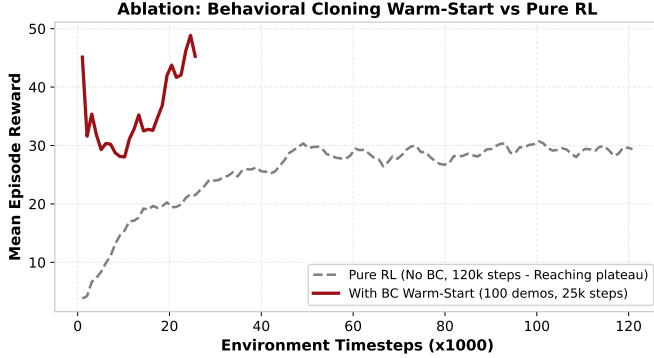
Figure 5. Behavior Cloning Warm-Start Ablation. BC initialization avoids the local reaching minimum and enables PPO to achieve stable lifting in only 25k steps.
