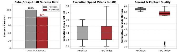
Figure 6. Empirical comparison between the Deterministic Heuristic FSM controller and the learned PPO policy during cube manipulation rollouts.
