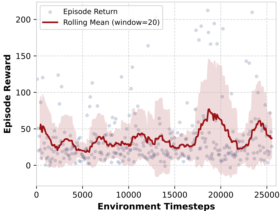
Training Reward Evolution
