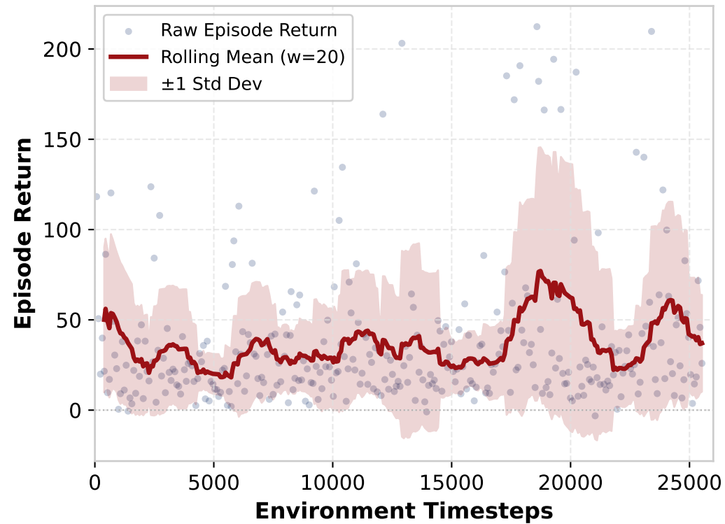
PPO Training Return Evolution
