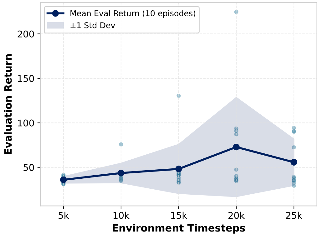
Periodic Policy Evaluation (Greedy)
