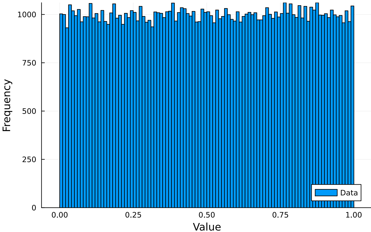
Histogram of Uniform(0,1) Data
