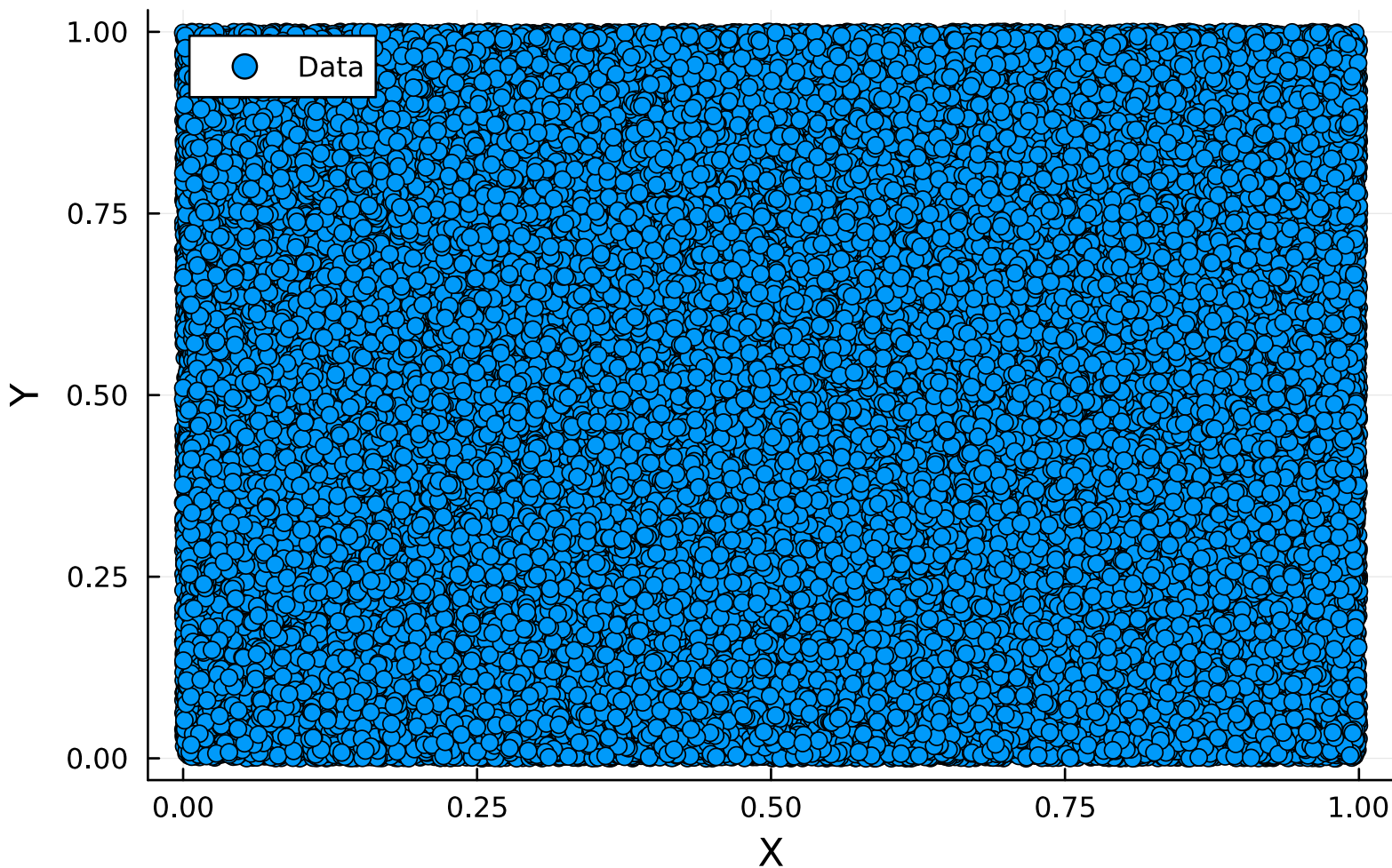
Scatter Plot of Uniform(0,1) Data
