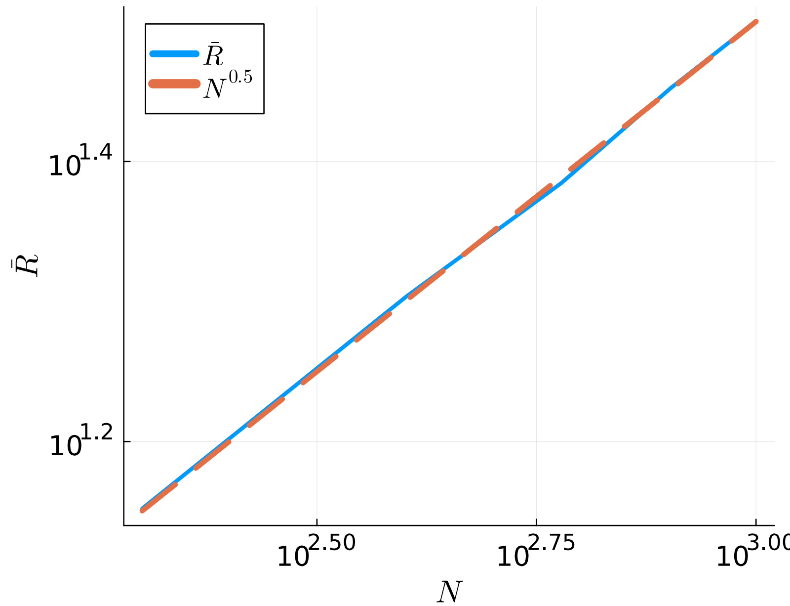
Random walk running 10000 times
