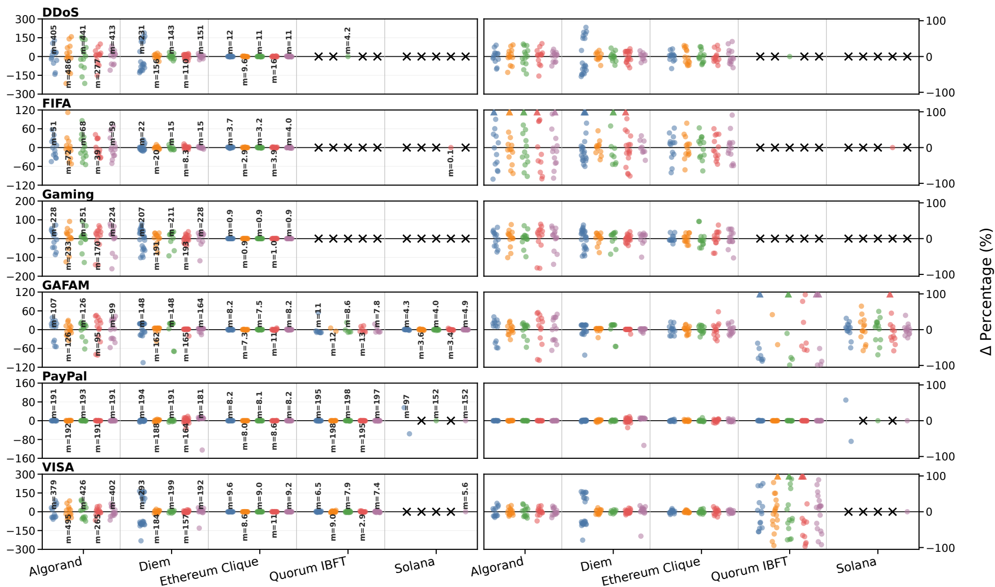
(b) Throughput deviations, 40 nodes, six workloads
