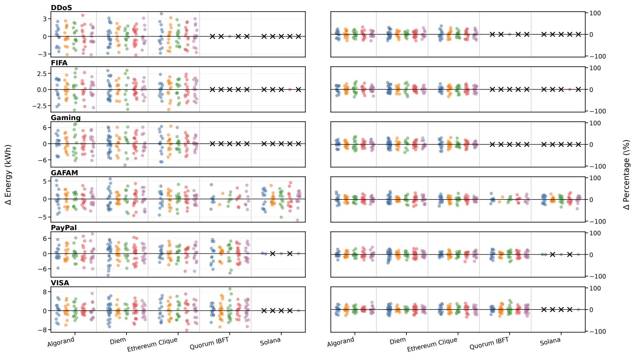
(b) Energy deviations, 40 nodes, six workloads
