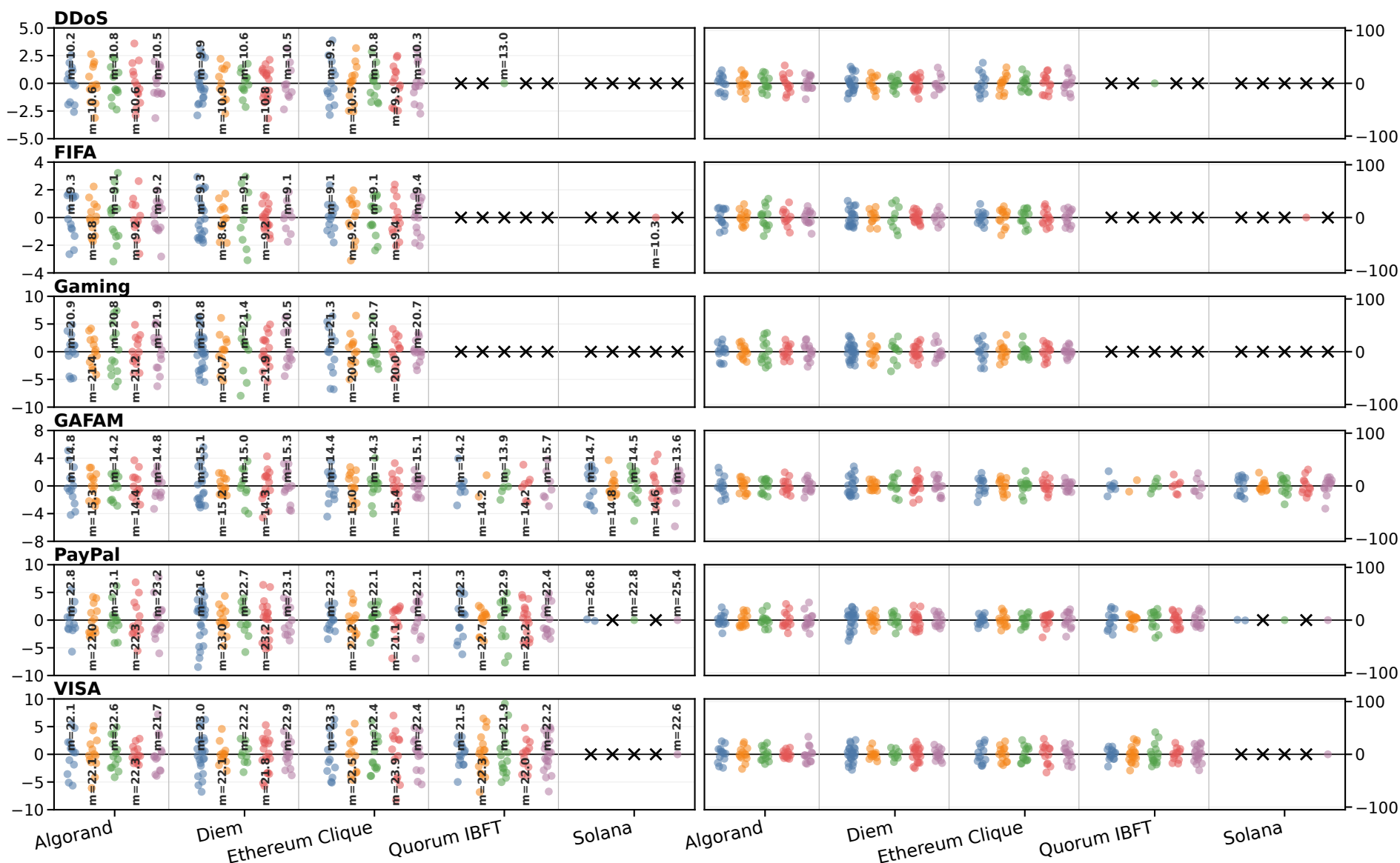
(b) Energy deviations, 40 nodes, six workloads
