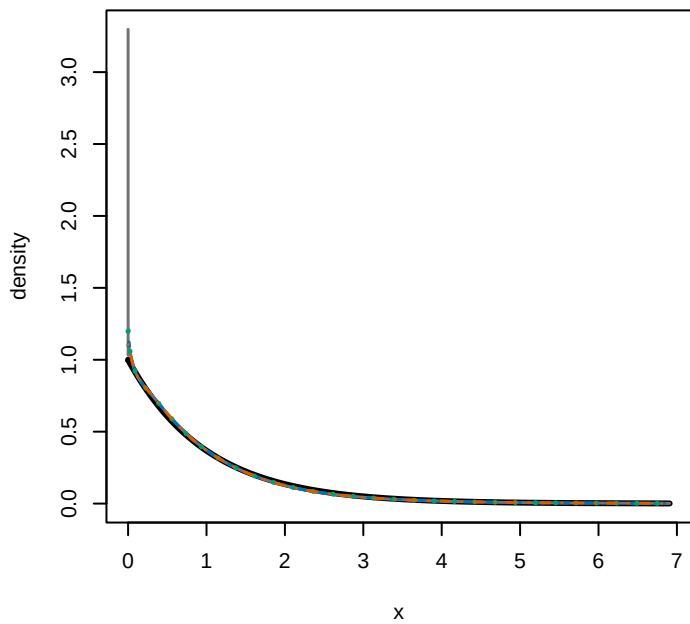
exponential, n=1000
