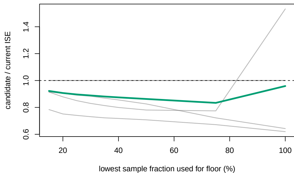
boundary ISE, n=1000
