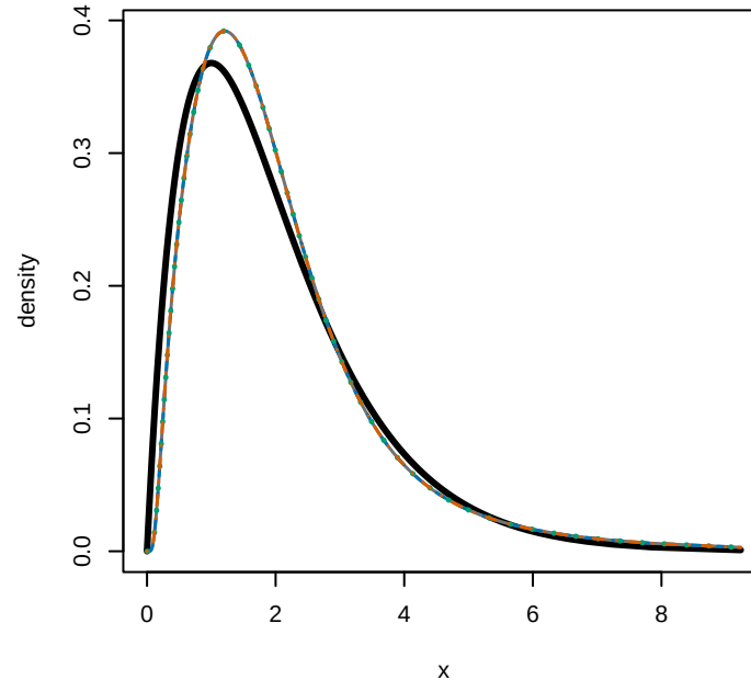
gamma_2, n=1000
