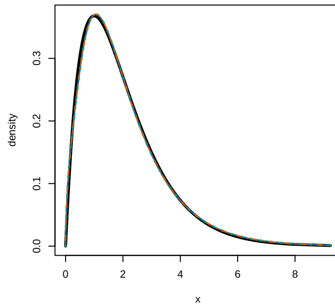
gamma_2, n=1000
