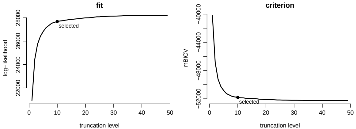
Figure 3: Log-likelihood and modified BIC against truncation level for the returns data, obtained by truncating the untruncated fit at each level. The filled point marks the level chosen by trunc_lv1 = NA . The criterion continues to improve beyond it, for the reason given in the text.
