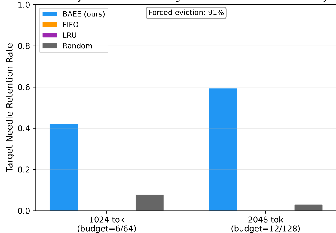
Memory-Pressure NIAH: Target Retention vs. Eviction Policy
