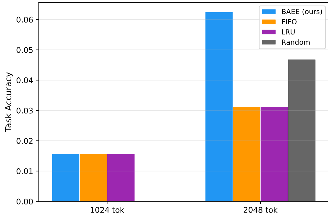
Memory-Pressure NIAH: Task Accuracy
