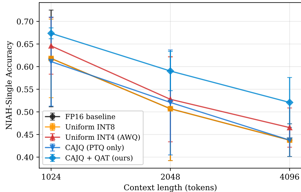
NIAH-Single Accuracy
