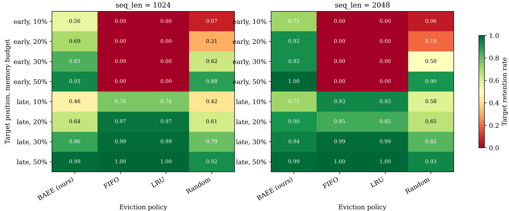
BAEE Grid: Target Retention Rate by Budget × Position × Policy
