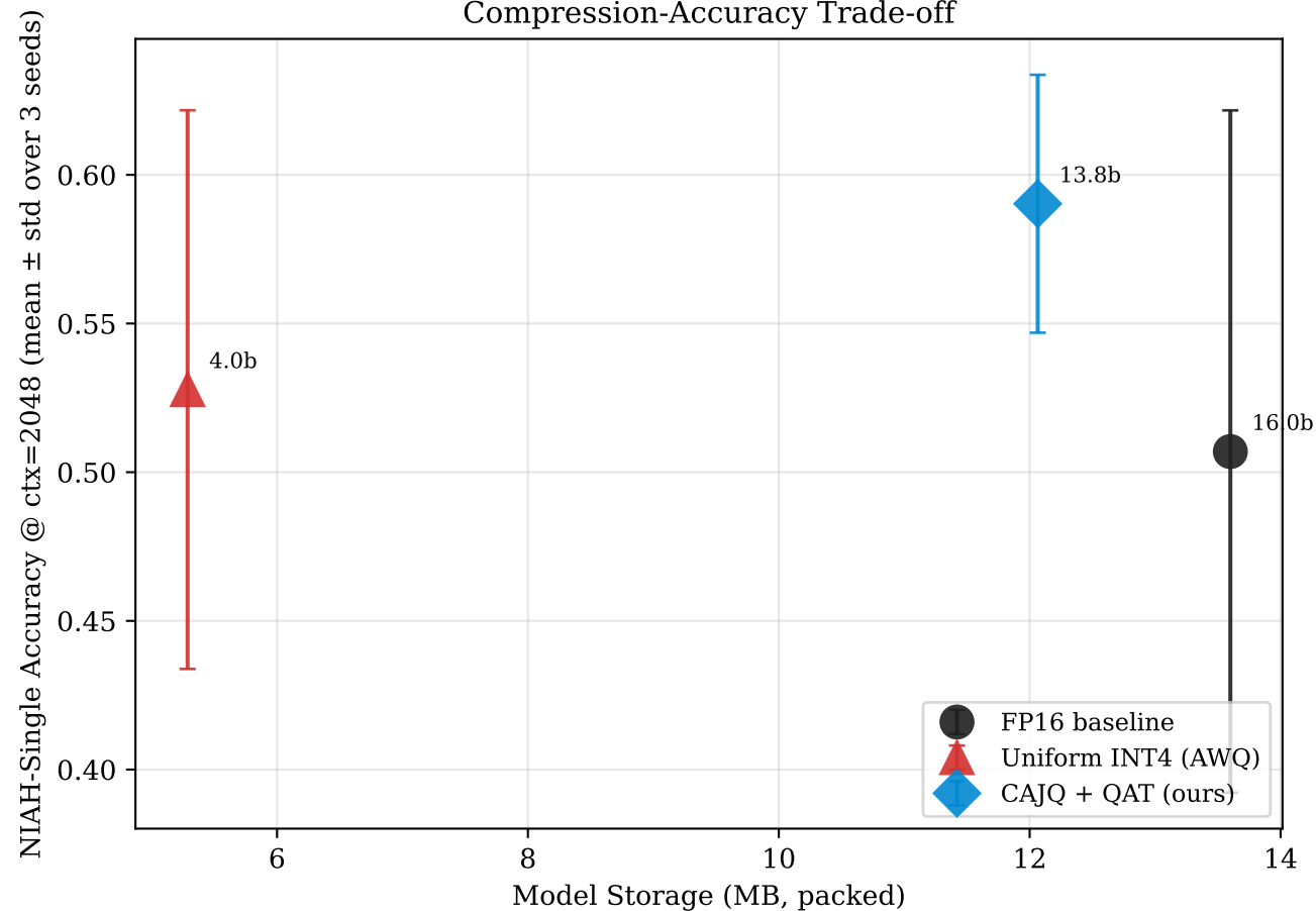
Compression-Accuracy Trade-off
