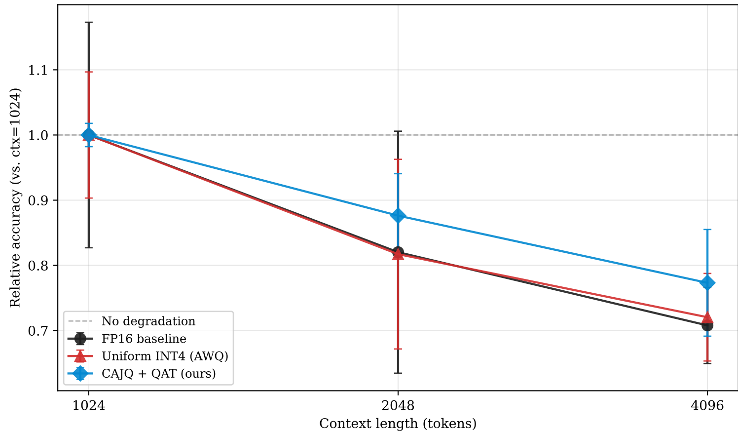
Long-Context Accuracy Degradation
