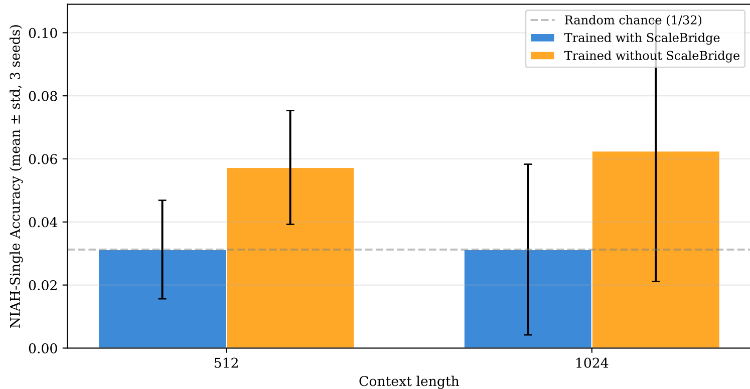
ScaleBridge from-scratch comparison (small-scale: dim=128, 400 steps)
