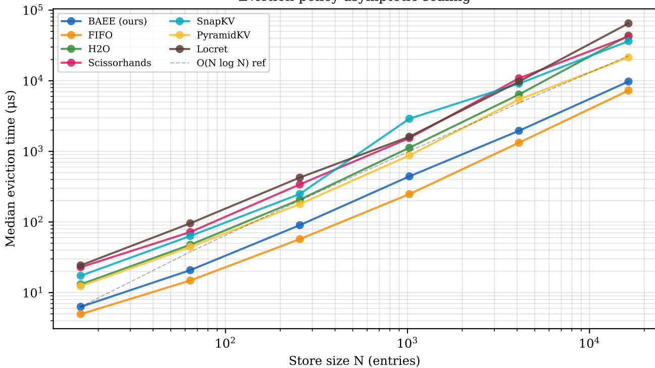
Eviction-policy asymptotic scaling
