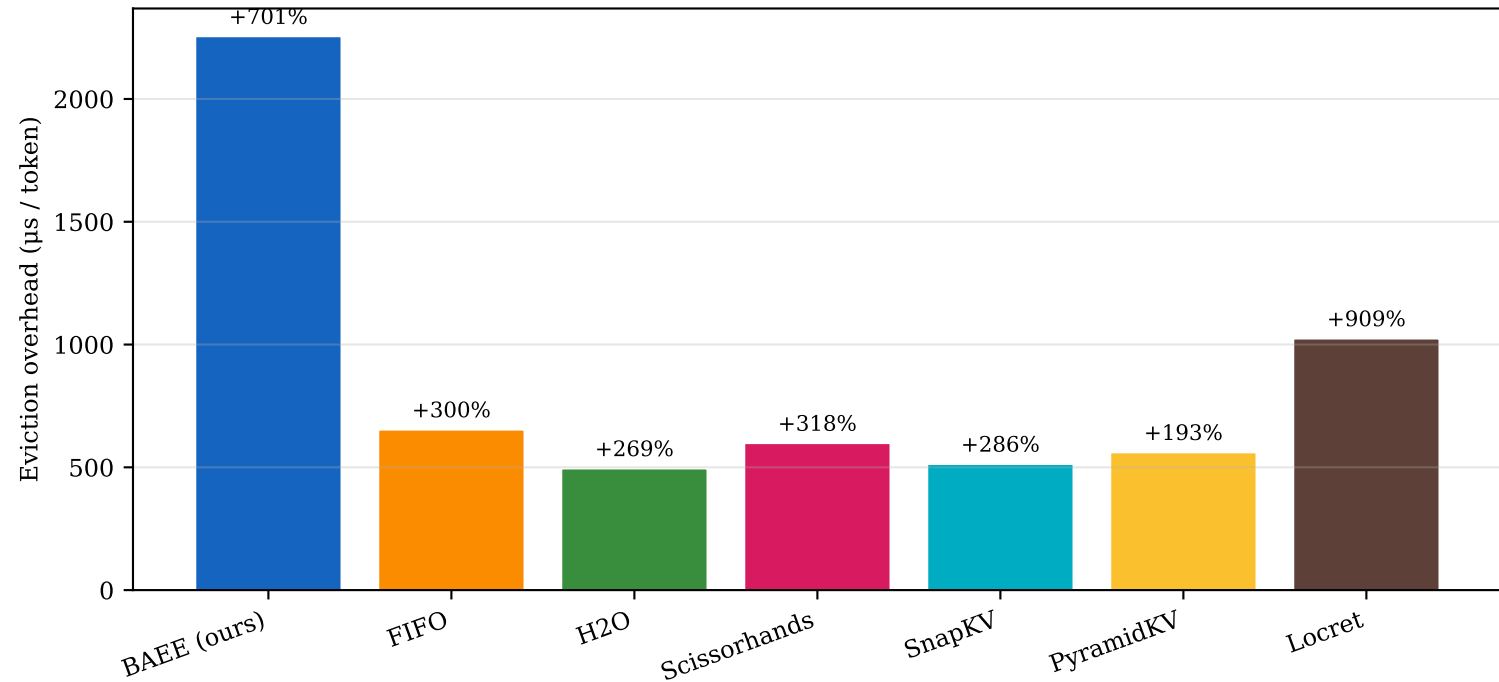
Per-token amortised eviction overhead (seq=2048, chunk=512, budget=32)
