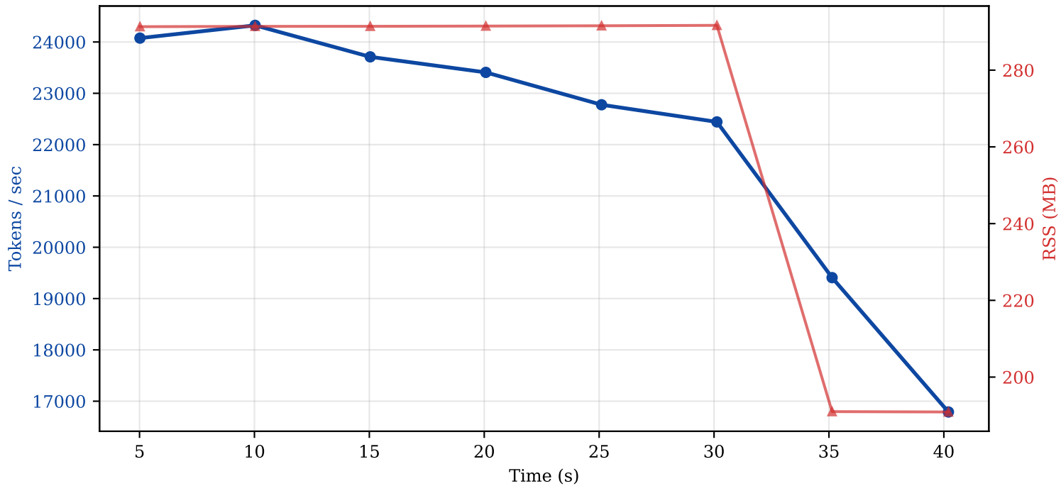
Sustained throughput stress test (45s, degradation = 30.3%)
