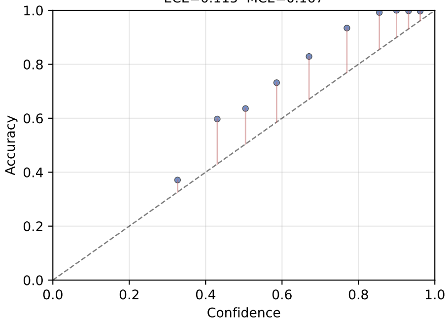
DINOv2 x Ordinal CapsNet ECE=0.115 MCE=0.167
