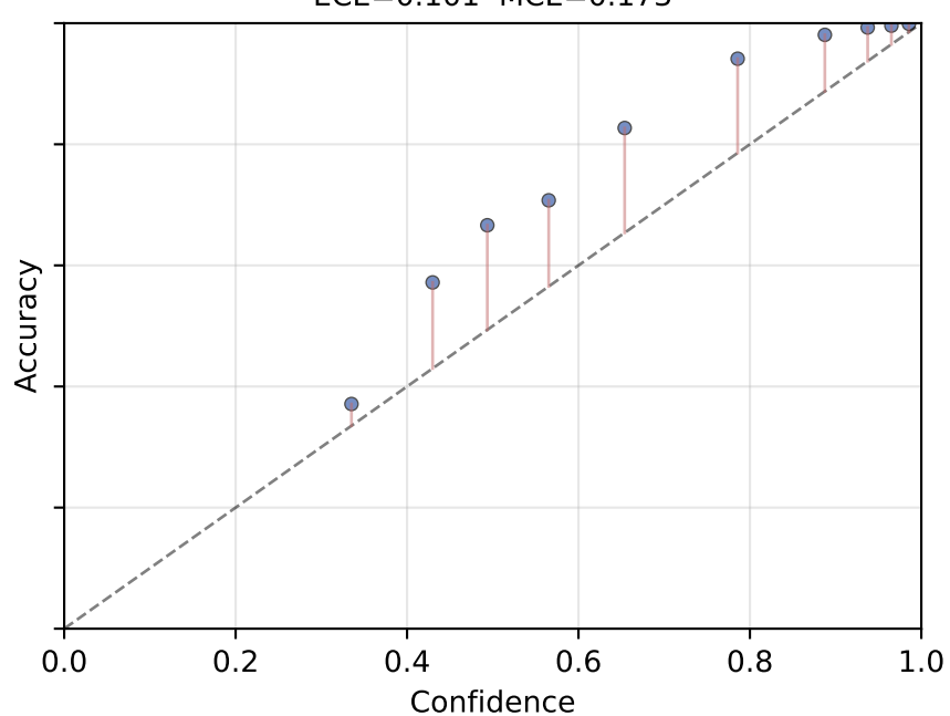
DINOv2 x MLP + K-1 sigmoid ECE=0.101 MCE=0.173
