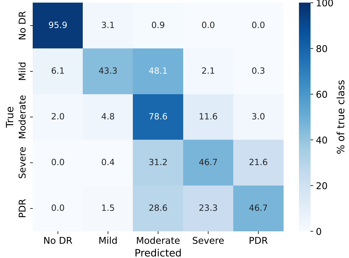
(b) Ordinal CapsNet
