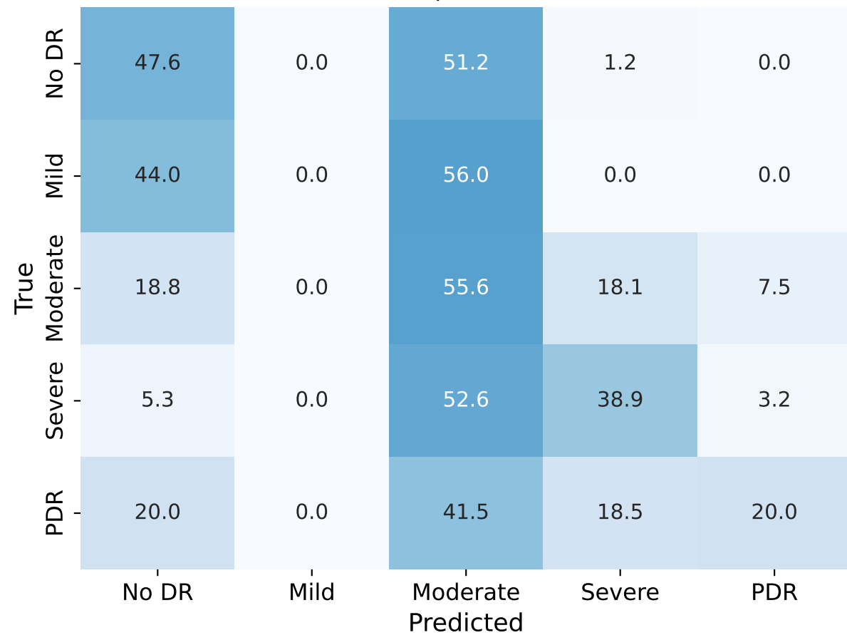
(a) Vanilla CapsNet (IDRiD test)
