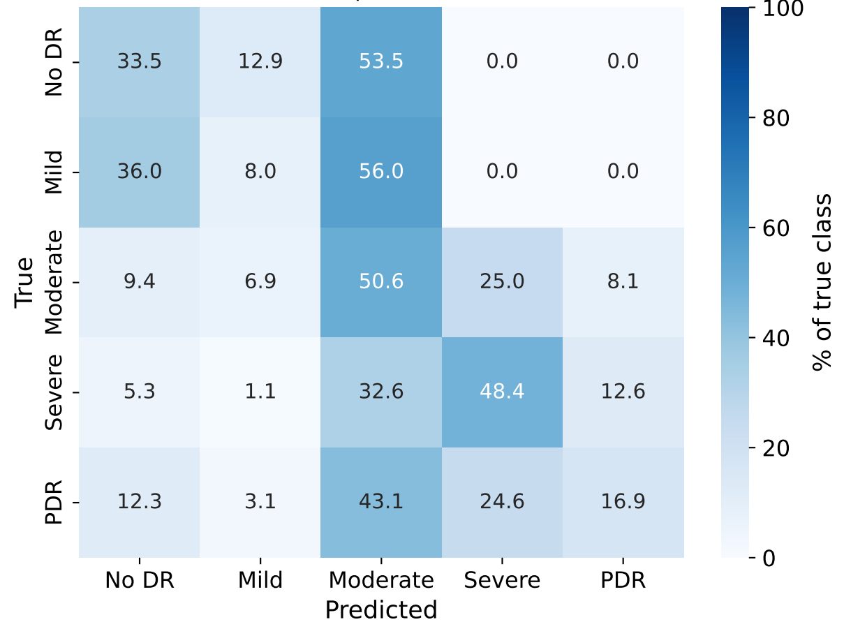
(b) Ordinal CapsNet (IDRiD test)
