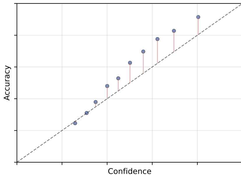
DINOv2 x MLP + K-1 sigmoid ECE=0.090 MCE=0.159
