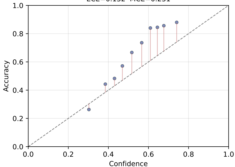
DINOv2 x Ordinal CapsNet ECE=0.132 MCE=0.231
