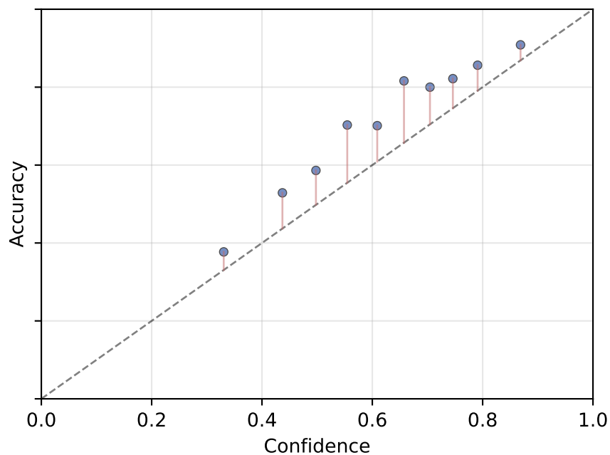
DINOv2 x MLP + K-1 sigmoid ECE=0.090 MCE=0.159
