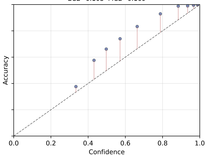
DINOv2 x MLP + K-1 sigmoid ECE=0.103 MCE=0.169
