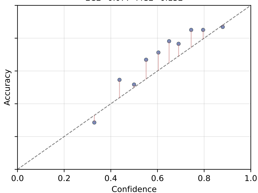
DINOv2 x MLP + K-1 sigmoid ECE=0.077 MCE=0.132
