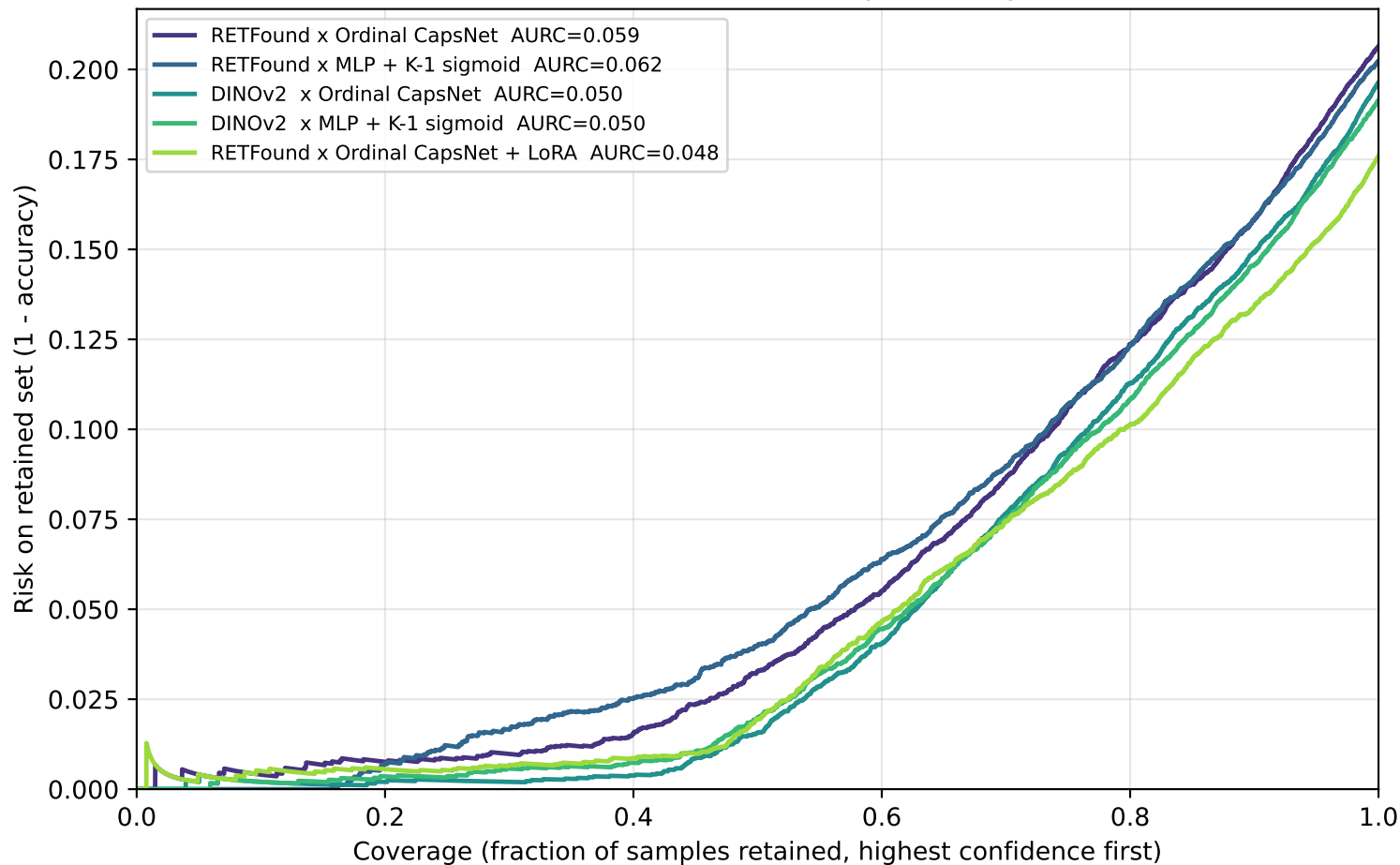
Risk-coverage curves on APTOS (selector: max chain-rule probability)
