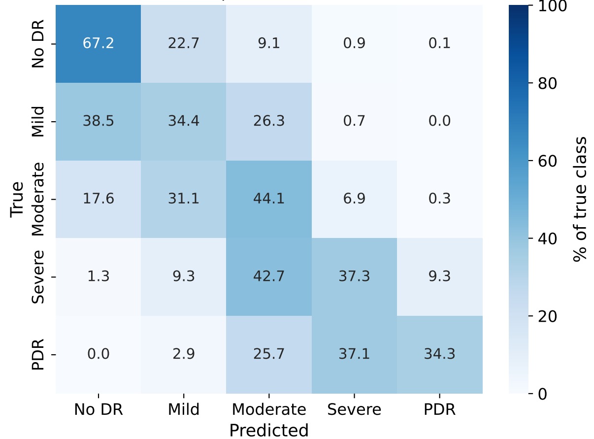
(b) Ordinal CapsNet (Messidor-2 within)
