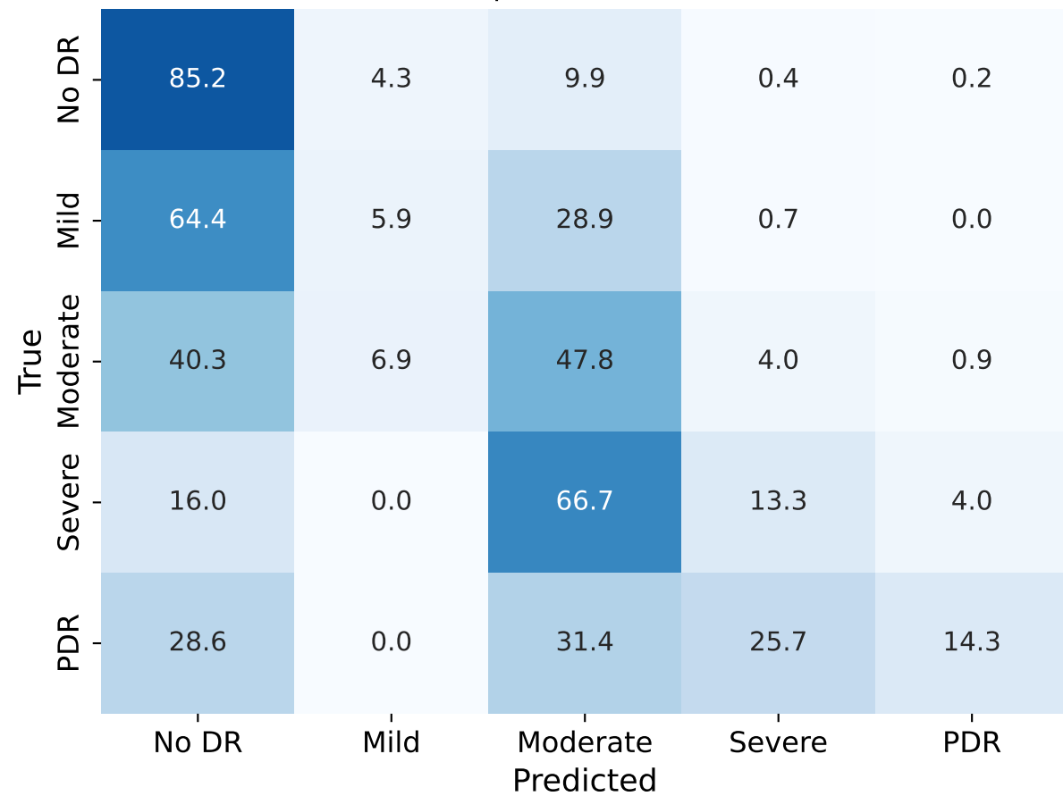
(a) Vanilla CapsNet (Messidor-2 within)
