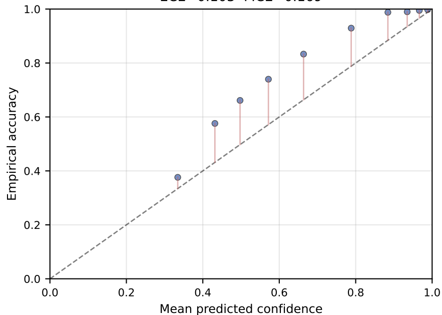
DINOv2 x MLP + K-1 sigmoid ECE=0.103 MCE=0.169
