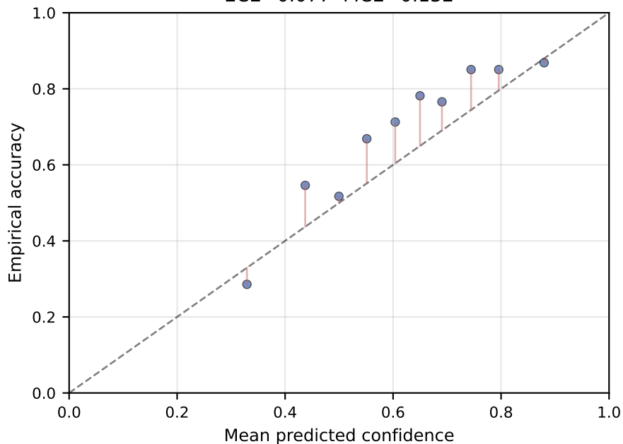
DINOv2 x MLP + K-1 sigmoid ECE=0.077 MCE=0.132
