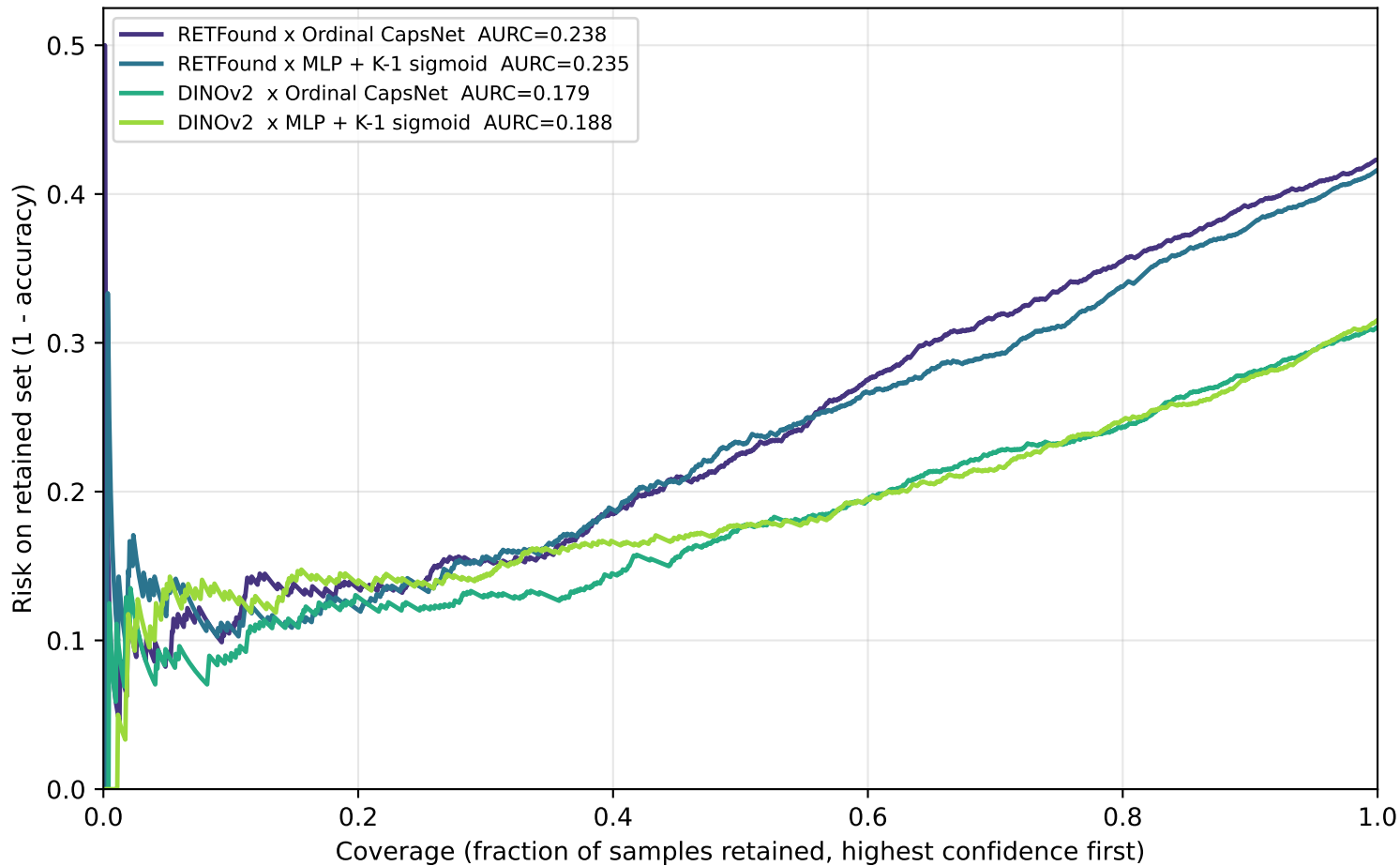
Risk-coverage curves on Messidor-2 (selector: max chain-rule probability)
