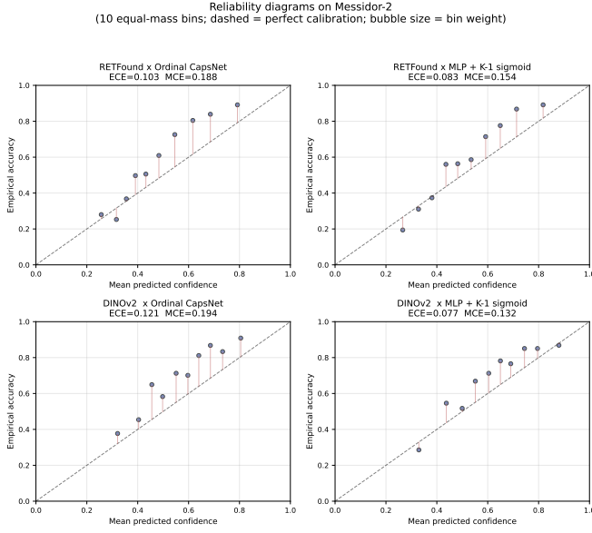
Fig. 5. Messidor-2 reliability diagrams for the four head×backbone cells.
