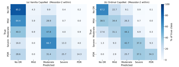
Fig. 4. Messidor-2 confusion matrices (RETFound backbone): Vanilla CapsNet (left) vs Ordinal CapsNet (right), pooled across 5 folds.
