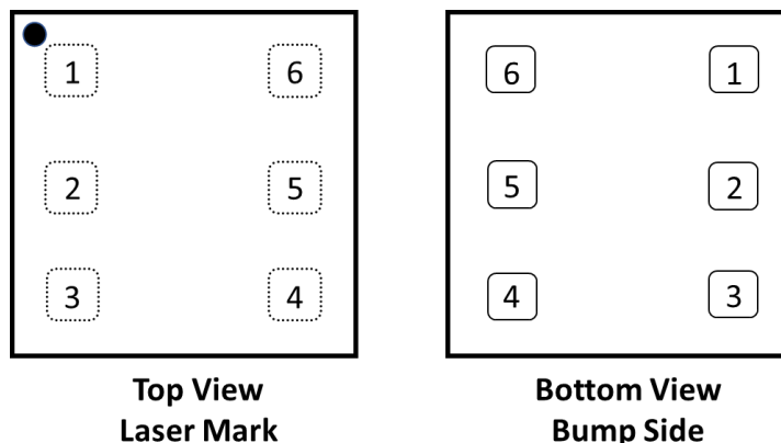
Figure 1: Pin Configuration
