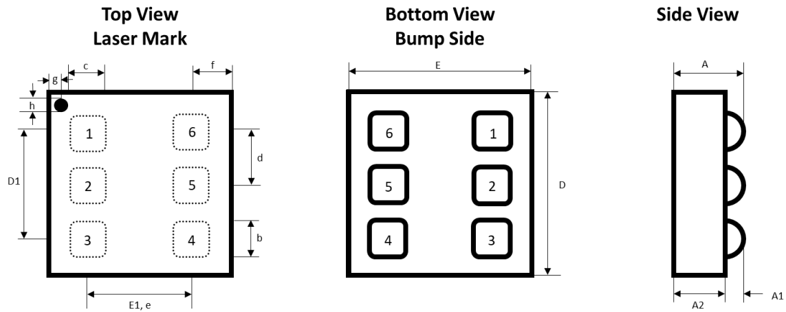
Figure 9: Package Dimensions
