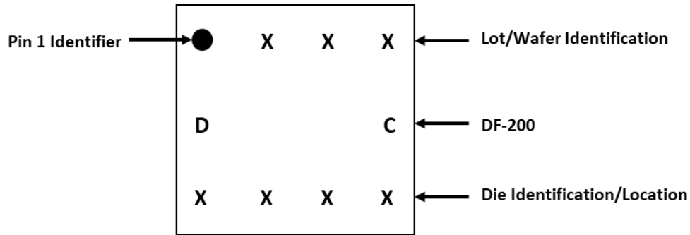
Figure 10: Top Mark
