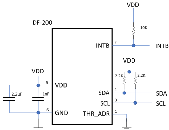
Figure 2: Typical Circuit for Button Application
