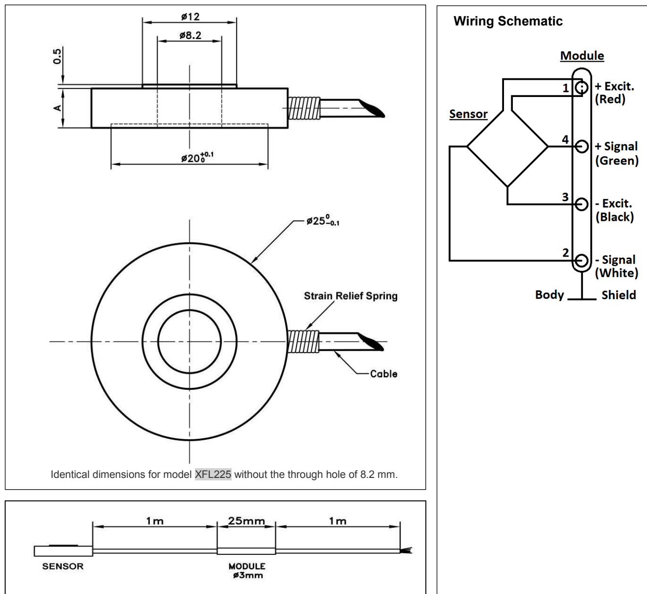
Dimensions in mm [inch]
