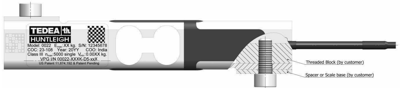
Mounting Configuration II
