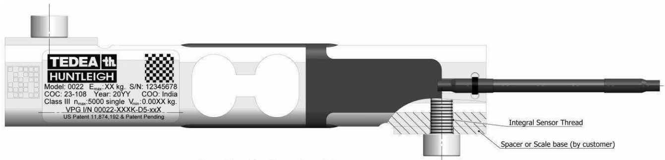
Mounting Configuration III
