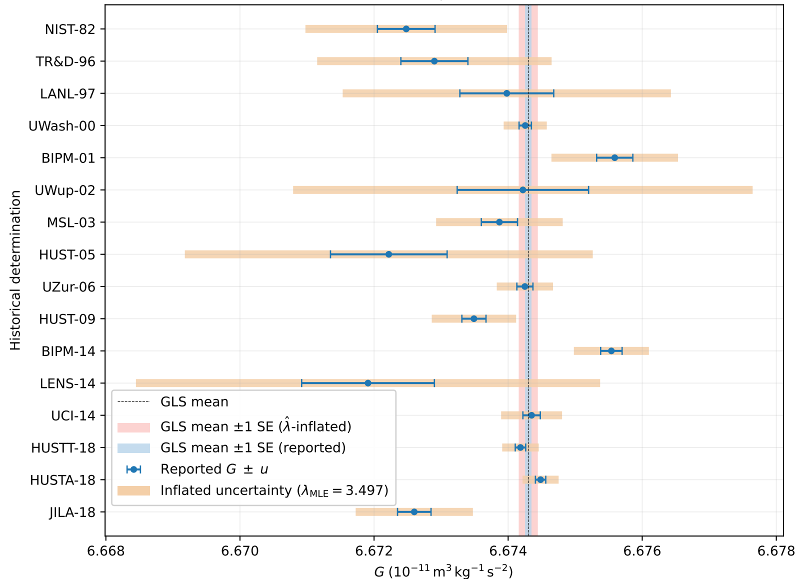
Historical determinations with quoted and inflated uncertainties
