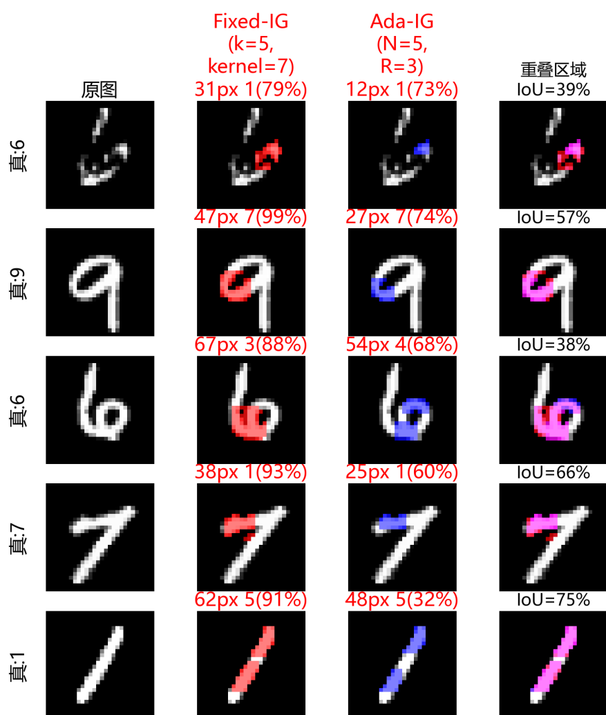
图 4.24 PGD-AT 模型: Fixed-IG vs Adaptive-IG 遮蔽位置对比 (参数 k = N = 5 , R = 3 , kernel = 7)
