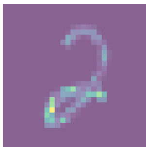
IG (n_steps=50) (Standard)
