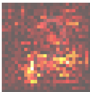
Saliency (Standard)
