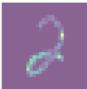
IG (n_steps=50) (PGD-AT)
