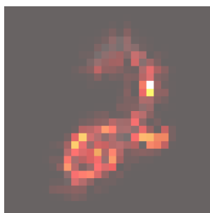
Saliency (PGD-AT)
